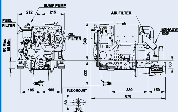
MODEL BETA 25
